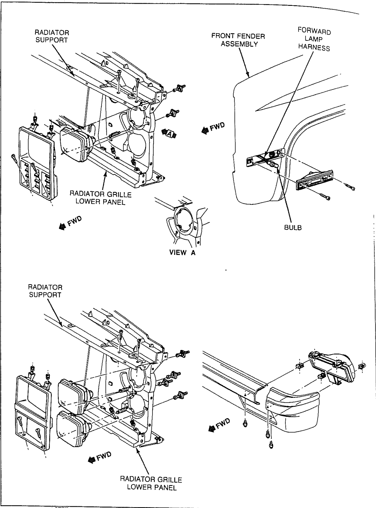
Fig. 8B-9--Front lighting (C-K Models)
